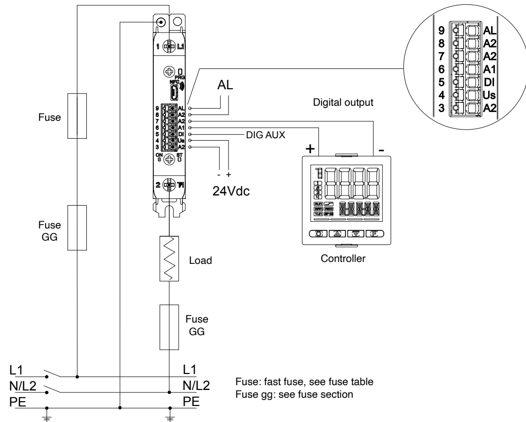
Connection for single phase load
